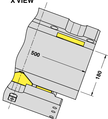
X VIEW
